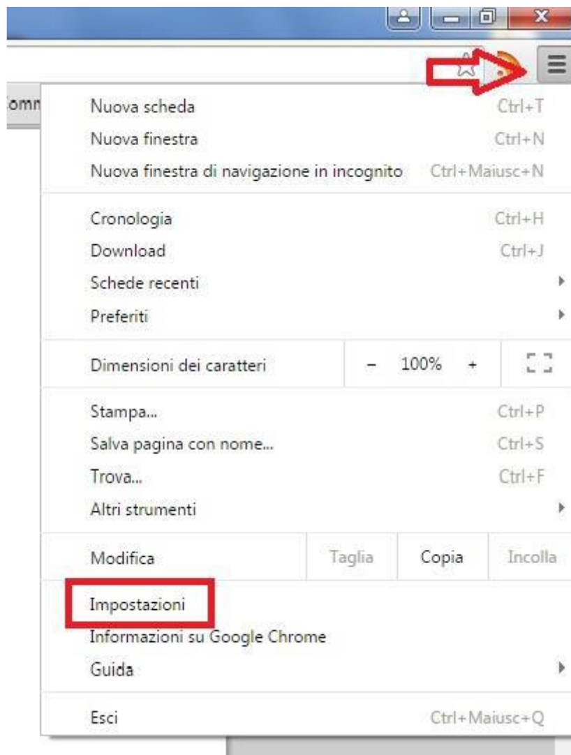
Figure 1 – Settings.
