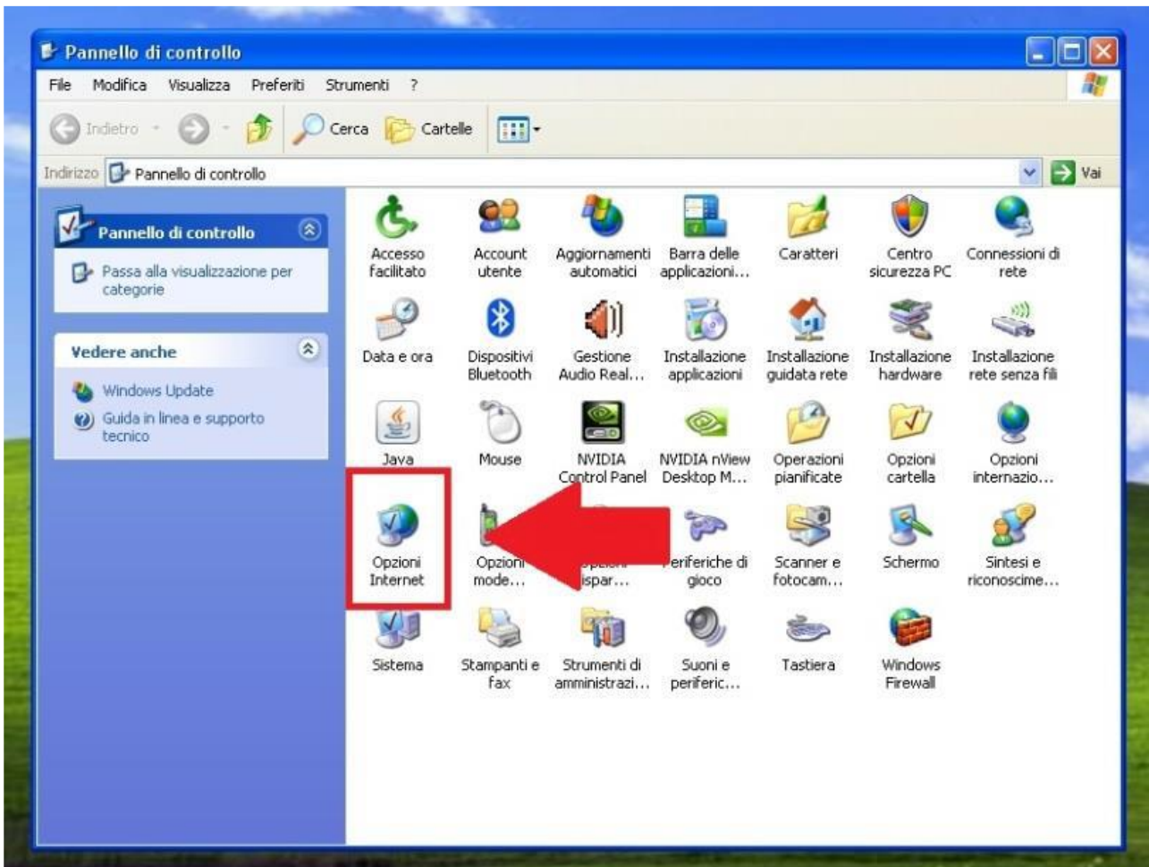
Figure 2 - Internet options.
