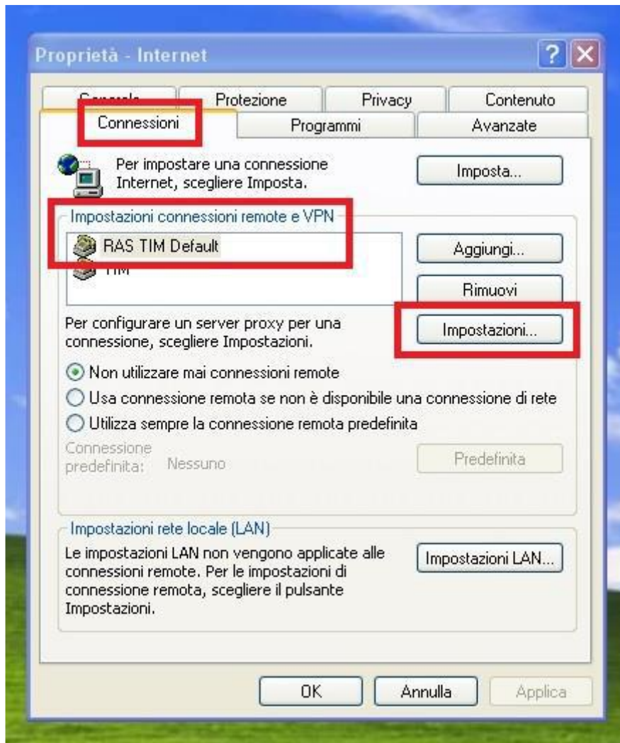
Figure 3 - Connections tab.
