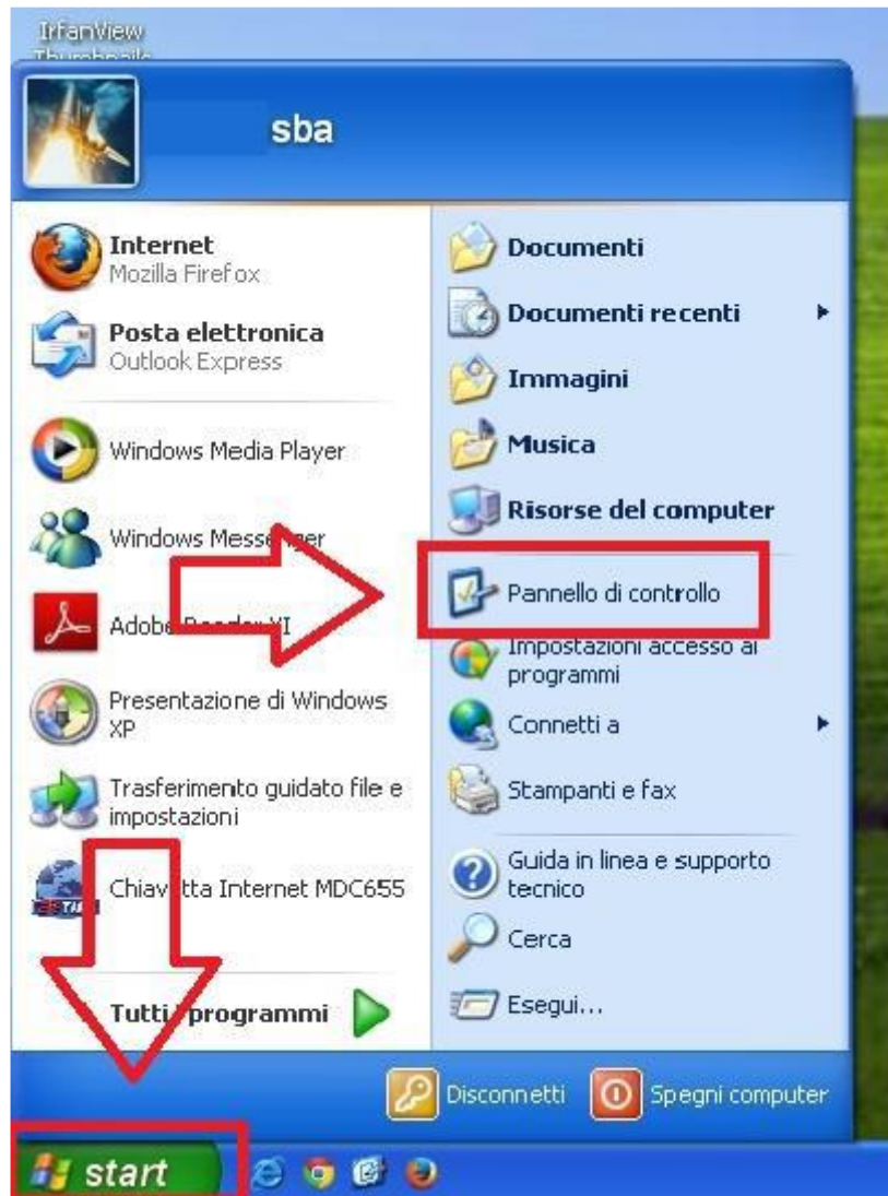
Figure 1 - Control panel
