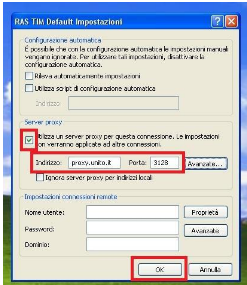
Figure 4 - Network settings.
